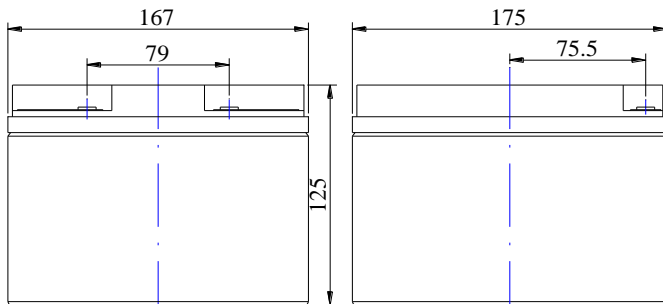
Battery bank spacing required 12.5mm (1/2"inch) minimum
