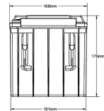
ODS-AGM70 RIGHT POSITIVE FEMALE TERMINALS
