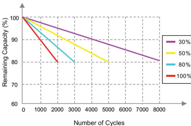
CYCLE LIFE CURVE AT 1C ACCORDING DOD
