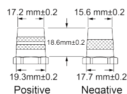
ODP-AGM25 LEFT POSITIVE SAE TERMINALS
