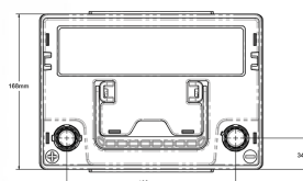
ODP-AGM25 LEFT POSITIVE SAE TERMINALS
